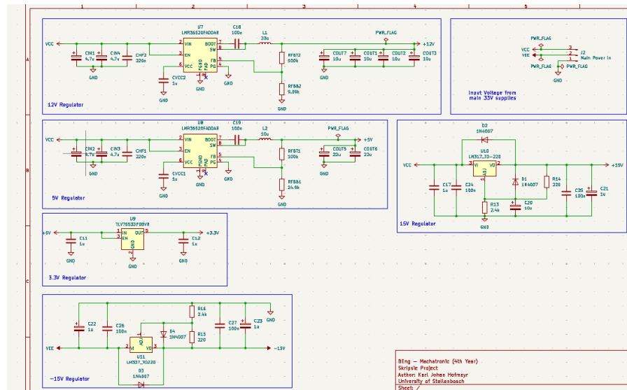
Figure 3: Voltage Regulator Circuits
