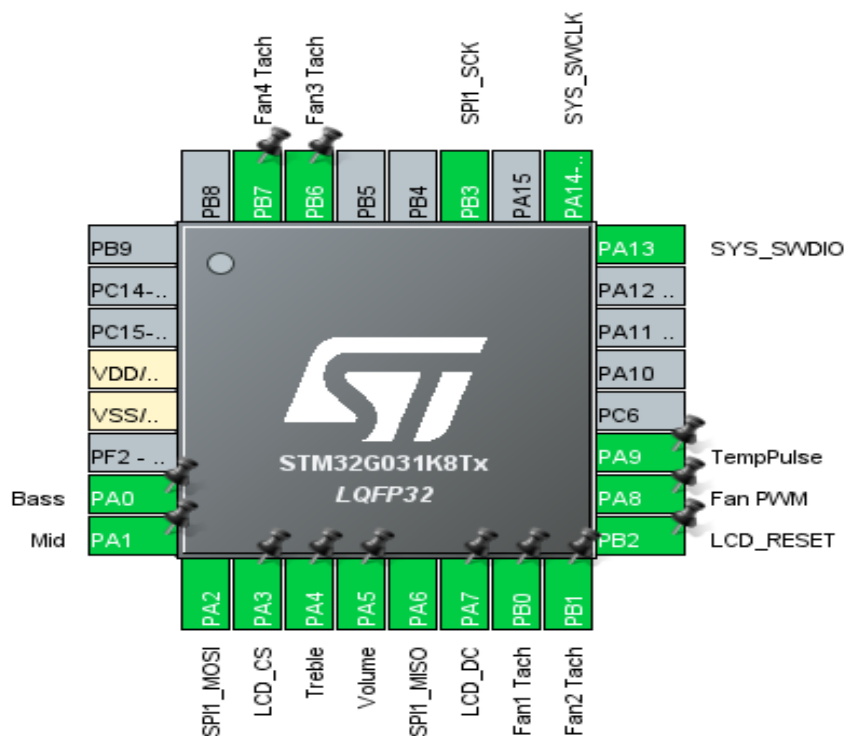
Figure 4: STM32 pinout setup
